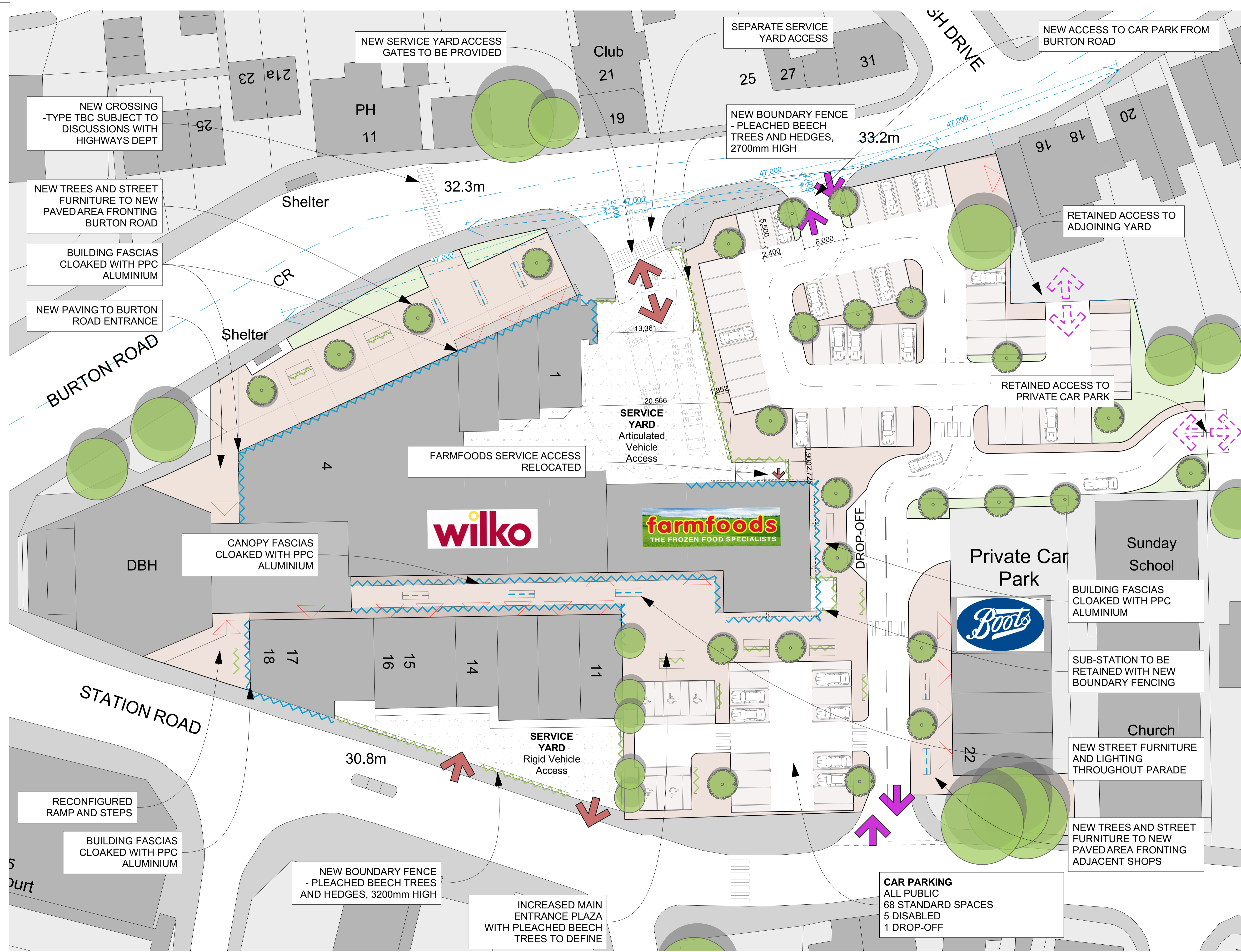
PROPOSED SITE PLAN - FEASIBILITY 1:250@A1
